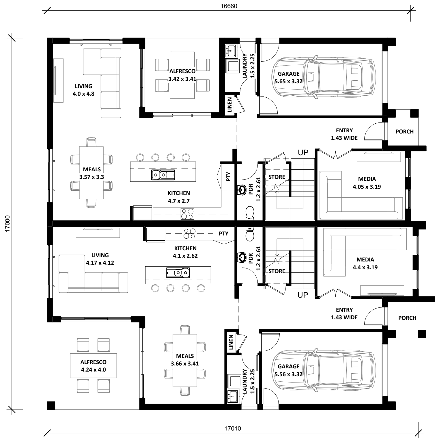
1 Ground Floor 1 : 100
