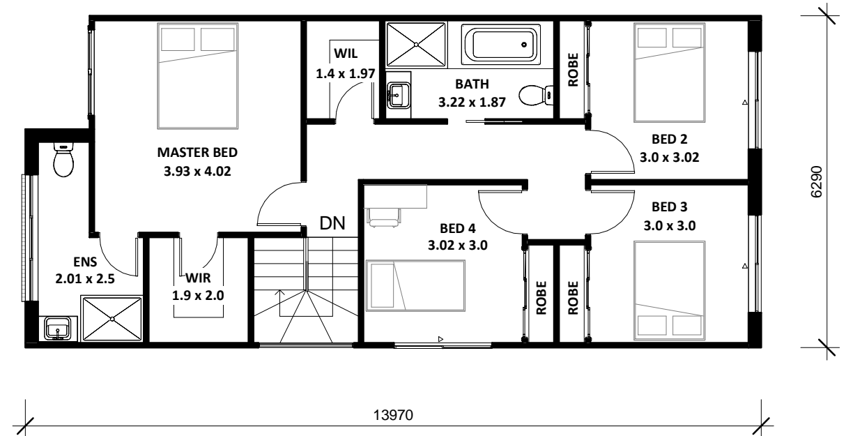
2 First Floor 1 : 100
