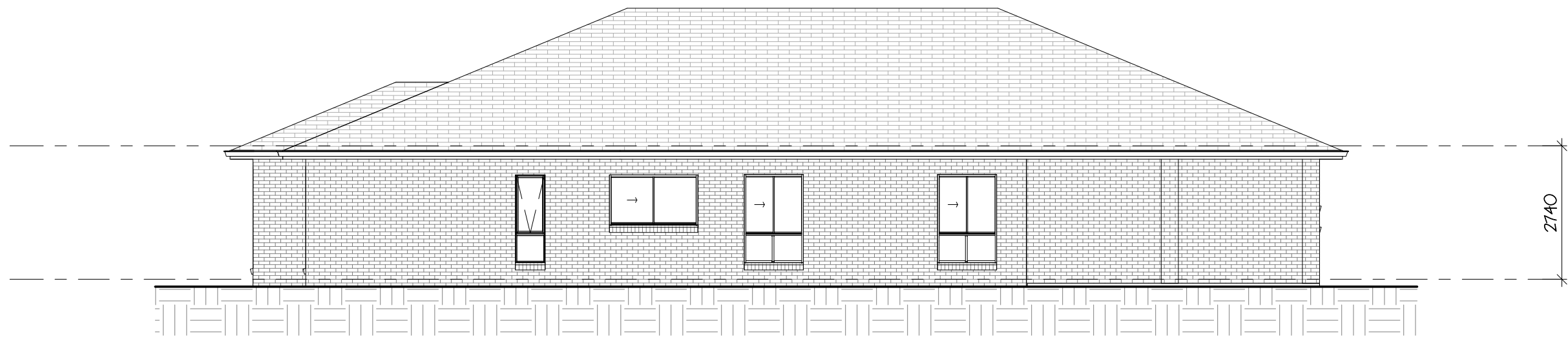
4 Right Side Elevation 1 : 100
