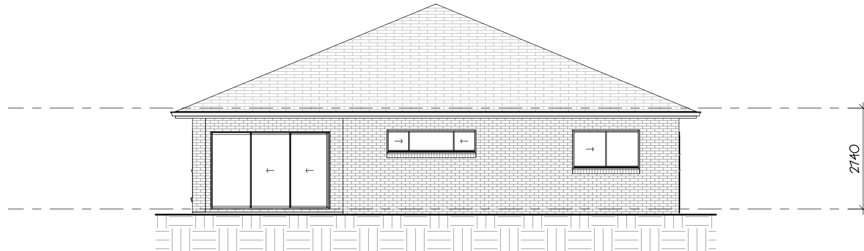
2 Rear Elevation 1 : 100
