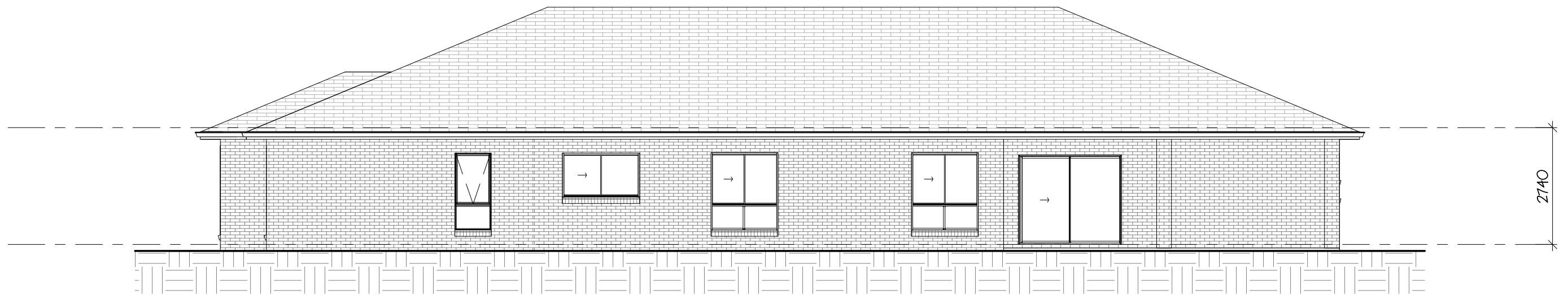
4 Right Side Elevation 1 : 100
