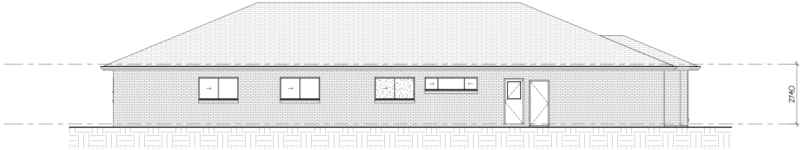
3 Left Side Elevation 1 : 100
