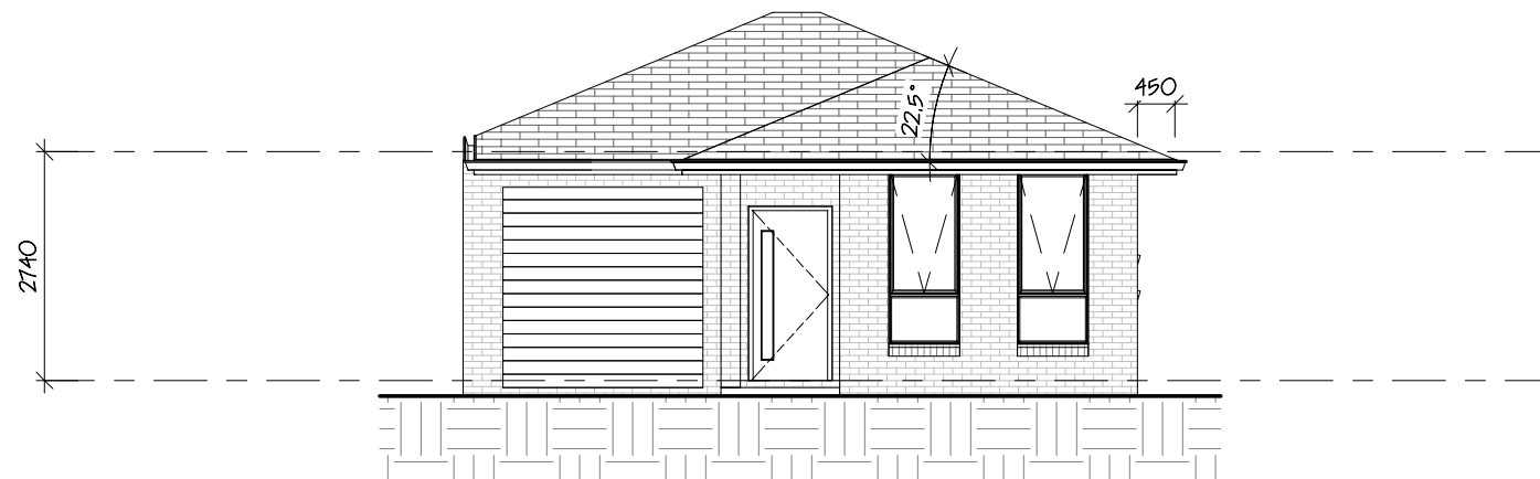
1 Front Elevation 1 : 100
