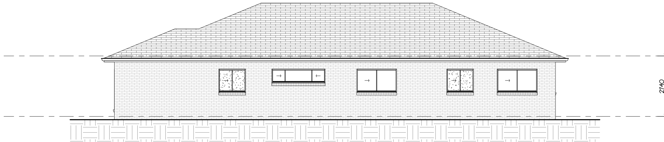
4 Right Side Elevation 1 : 100
