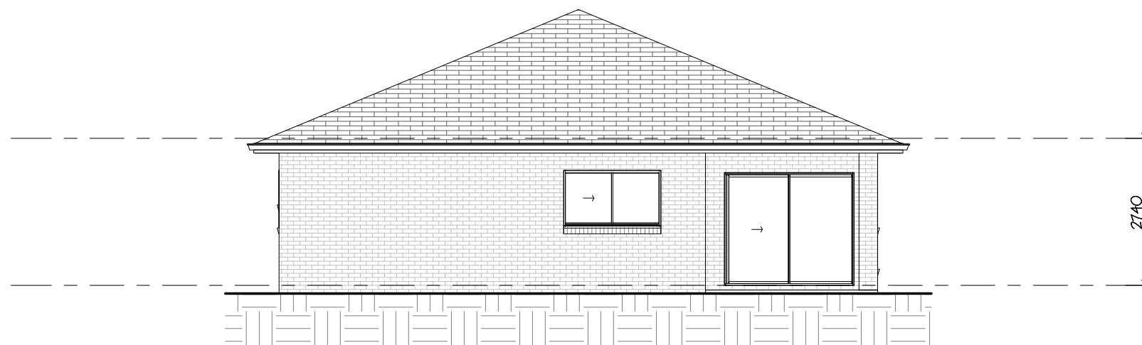
2 Rear Elevation 1 : 100
