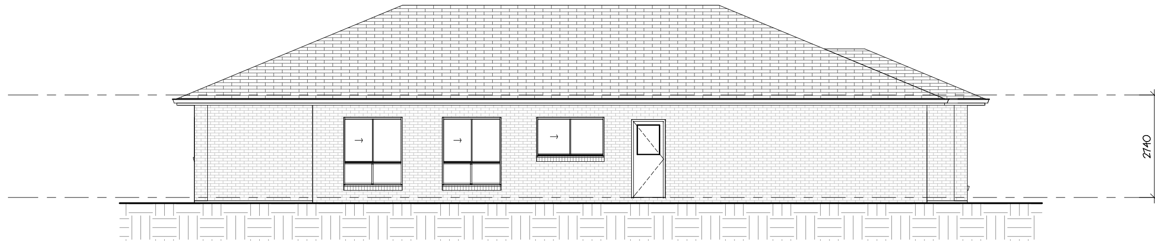
3 Left Side Elevation 1 : 100
